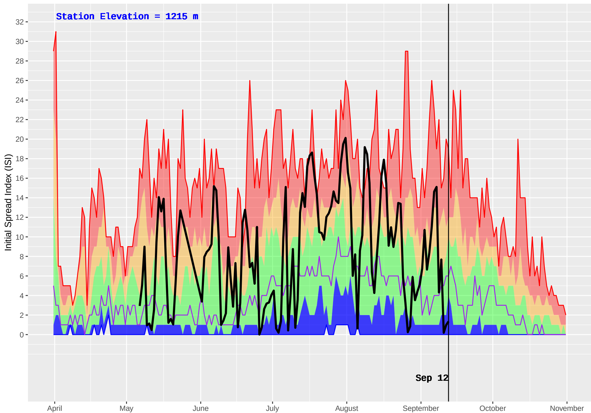
ALLISON PASS (317) : Historical (1987–2016) and Current (2018) Daily Initial Spread Index (ISI)
